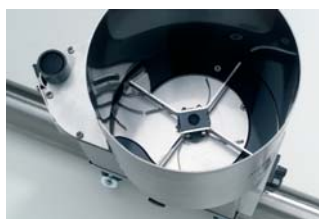
Storage container with double star wheel
